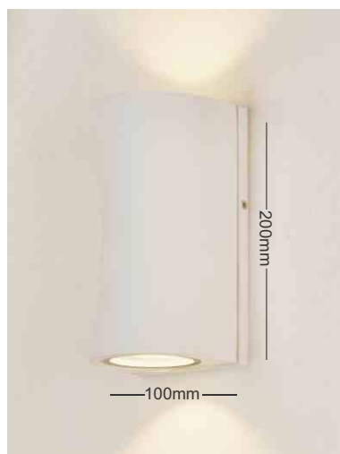
VC 1269S Ø100 L100 H200 Led 7w x 2 785.000đ
