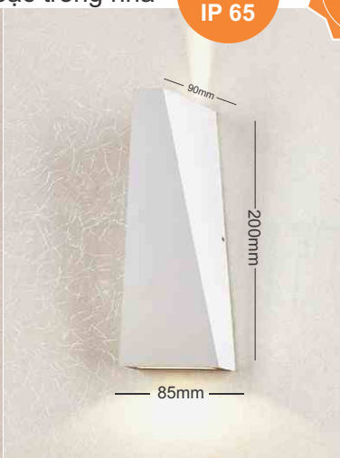
VC 1268S Ø85 L85 H200 Led 7w x 2 645.000đ
